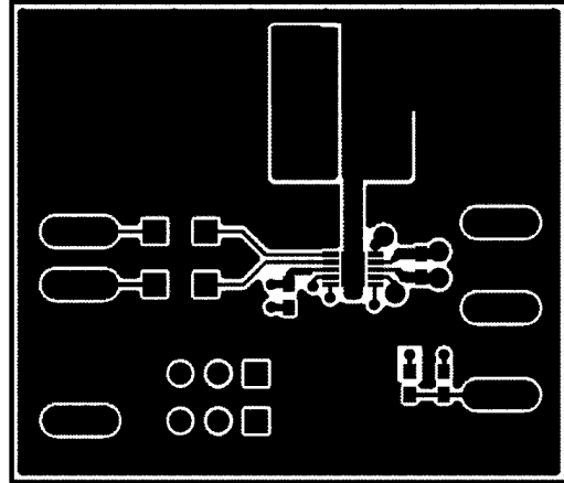
FIGURE 10. Top Layer
