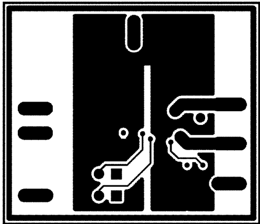
FIGURE 11. Layer 2 (GND)
