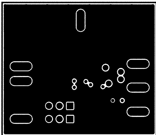
FIGURE 13. Bottom Layer
