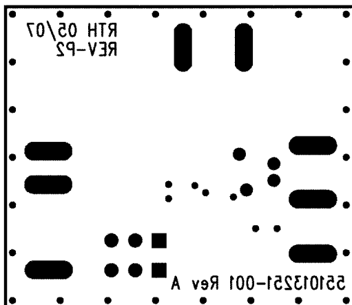
FIGURE 14. Bottom Silkscreen
